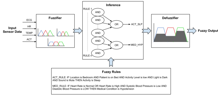
Fig. 1 A Fuzzy Logic System
